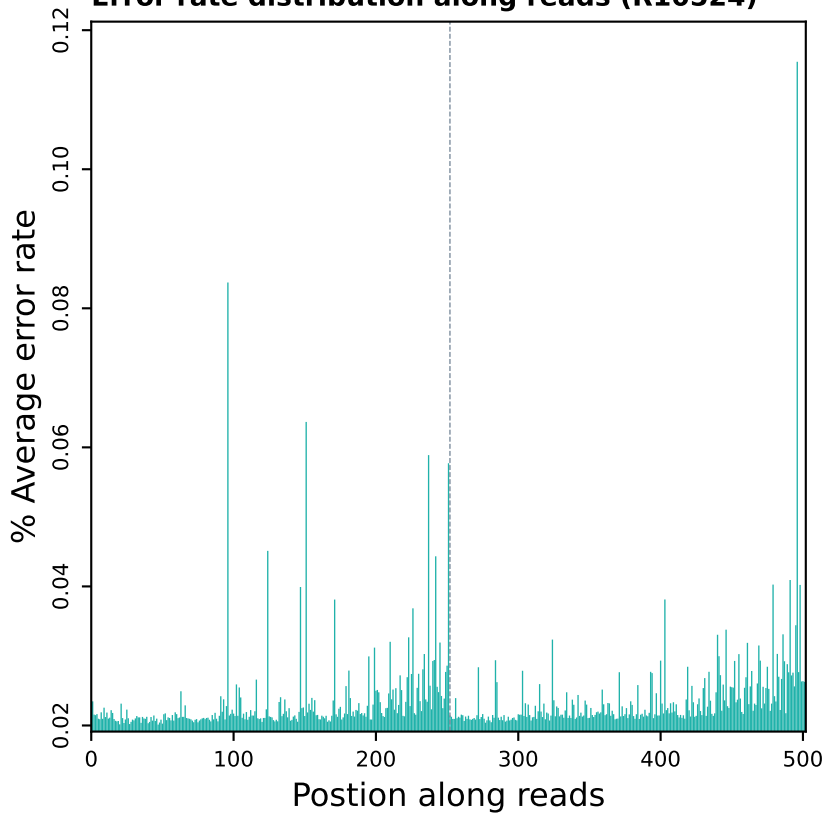
Error rate distribution along reads (R10524)
